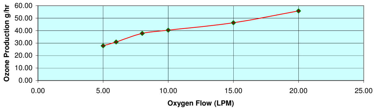
Ozone Production
