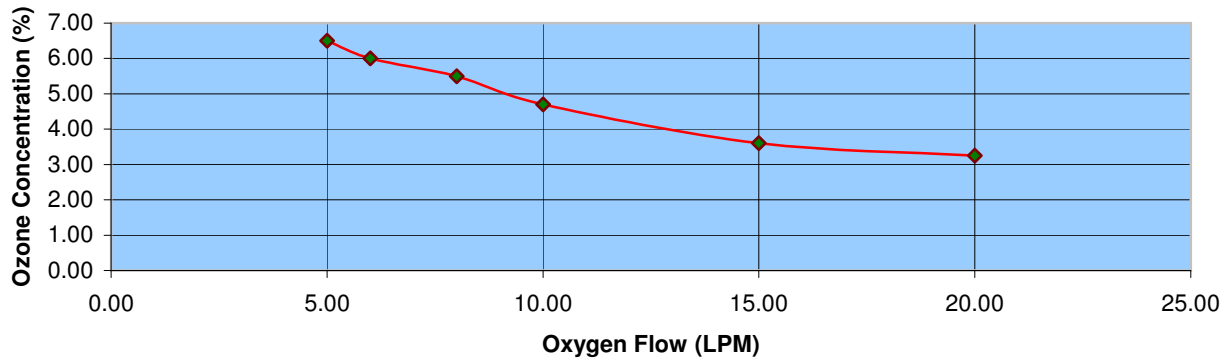
Ozone Concentration
