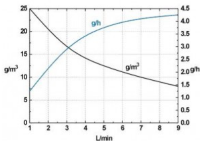
SR-8 Performance Chart on Dry Air
