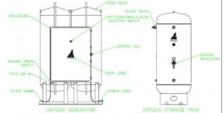
External System Diagram shows the OG-50 with the oxygen storage tank.
