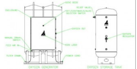
External System Diagram shows the OG-25 with the oxygen storage tank.
