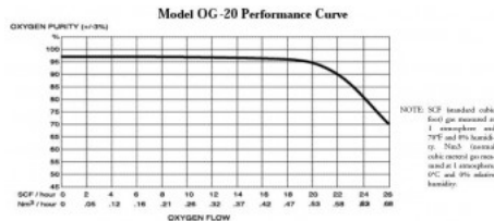
OG-20 Specifications
