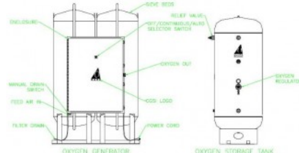
External System Diagram shows the OG-100 with the oxygen storage tank.
