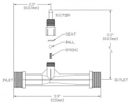
Drawing showing the dimensions of the MK-784 Ozone Venturi. Perfect for ozone installations for water treatment.
