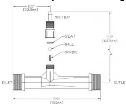
Drawing showing the dimensions of the MK-784 Ozone Venturi. Perfect for ozone installations for water treatment.
