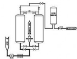
Process Diagram of the entire Oxygen Concentrating System
