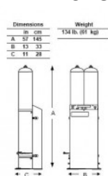
Dimensions of the AS-A Oxygen Concentrator
