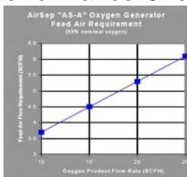
AS-A Performance chart
